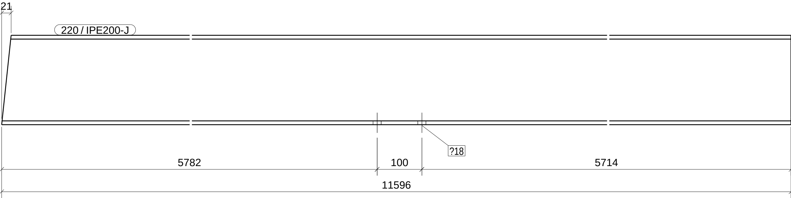
FRONT VIEW
